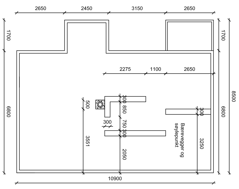
Betongplan
