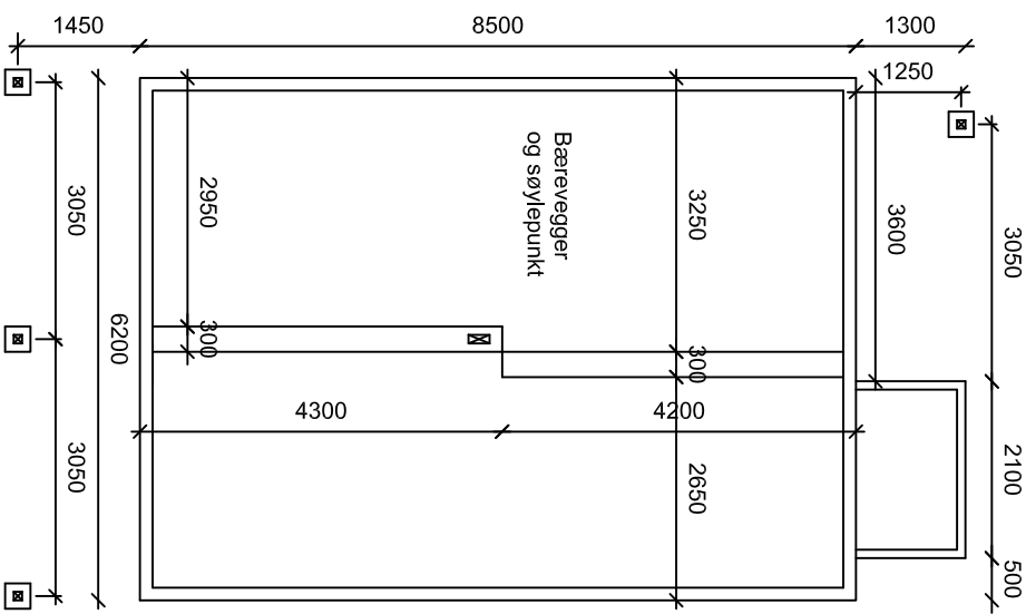
Betongplan
